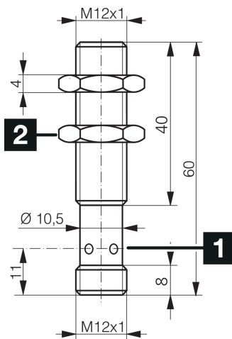
1) LED 4 x 90° (yellow) 2) Width over flats 17 mm BK: black BN: brown BU: blue
